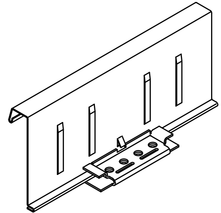
ASSEMBLED ISOMETRIC
