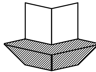
FORMED VIEW QC NOTE: NO SCRATCHES WITHIN HATCHED AREA
