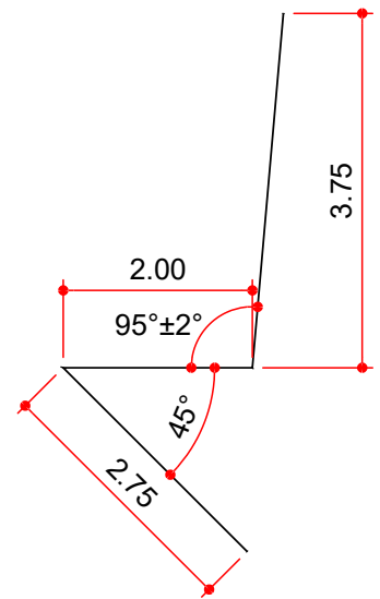
SIDE VIEW ALL ANGLES ARE ±3°
